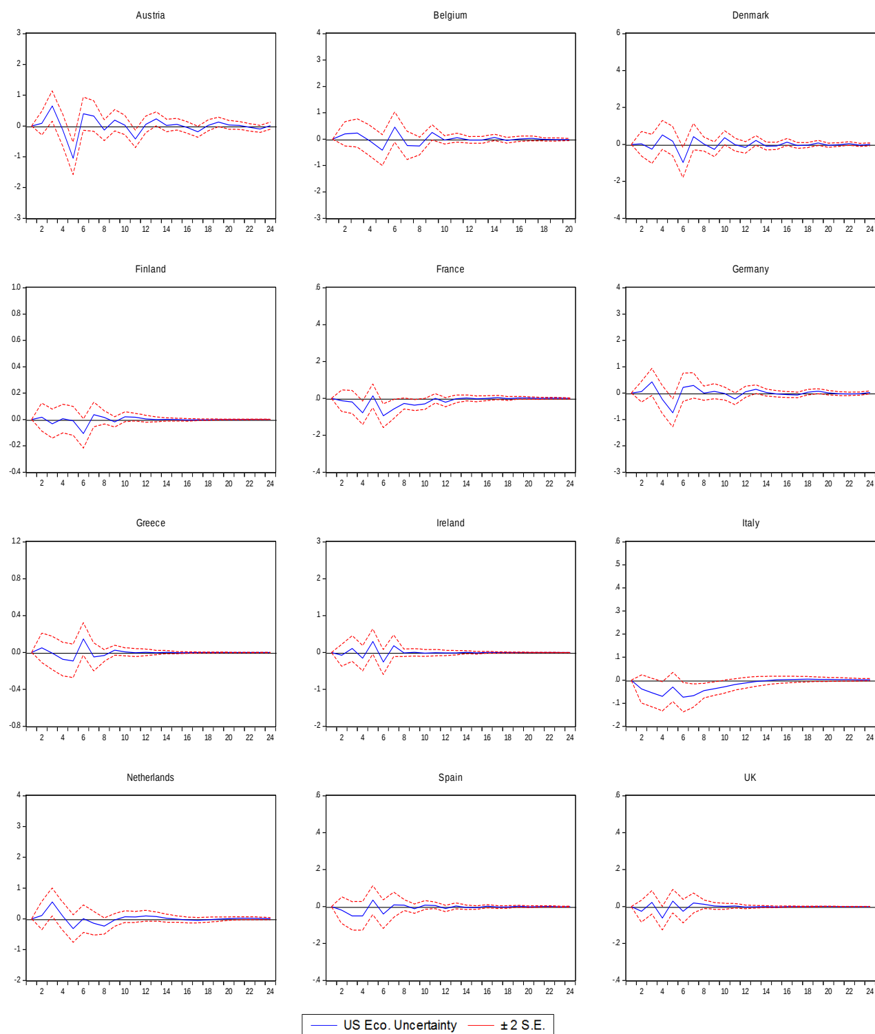
Figure 4 : Impulse Response Functions – Before Financial Crisis (Response of BC to Cholesky One S.D. Innovations in US Eco Uncertainty)
